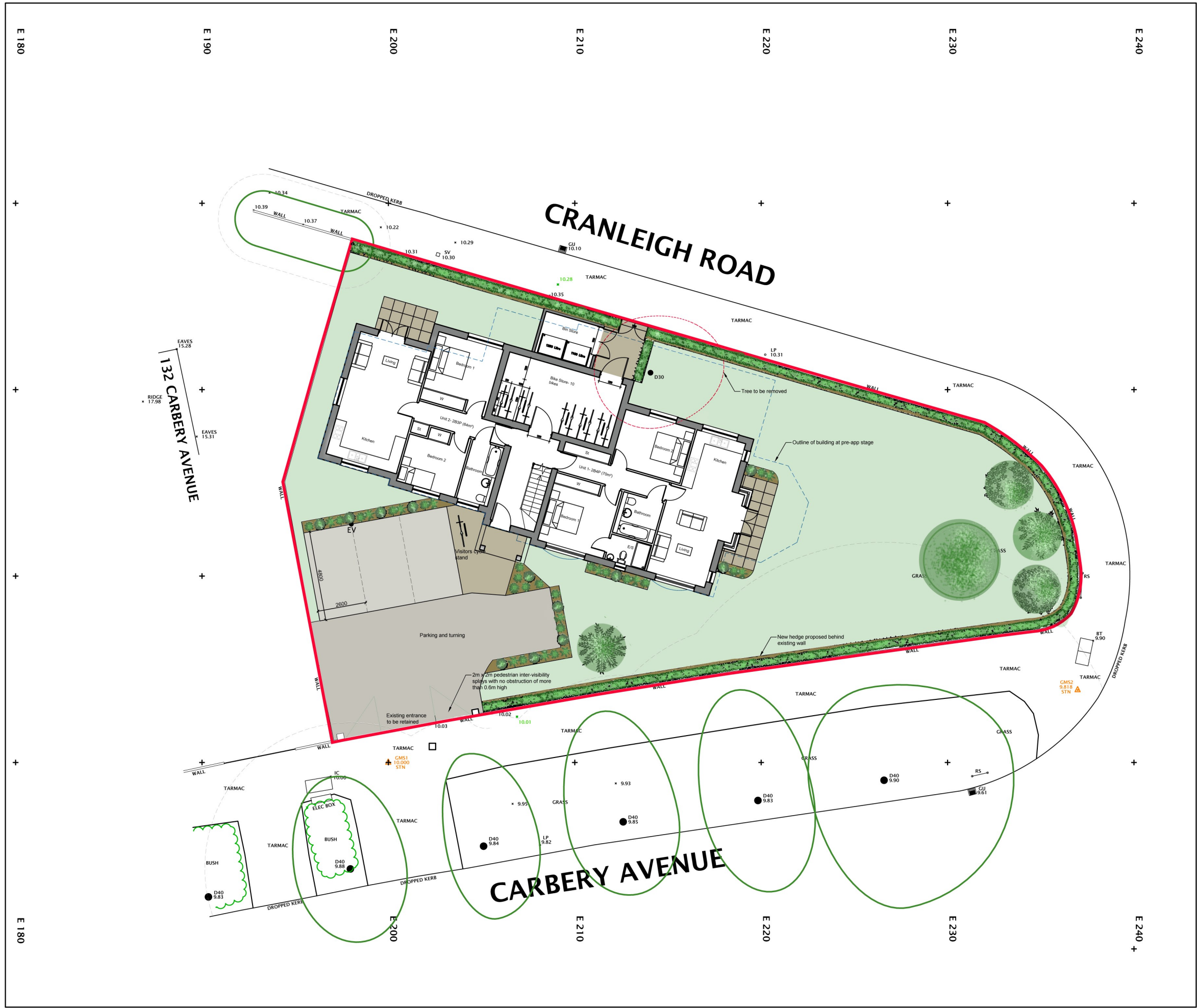
Proposed Site Plan 1:200 0 20m
